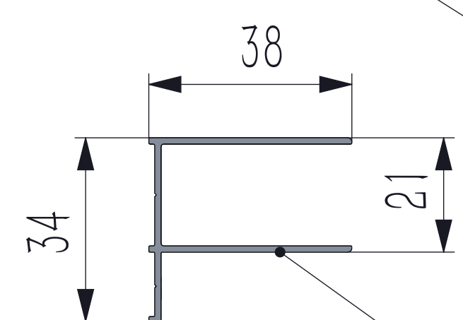
Glass Profile
